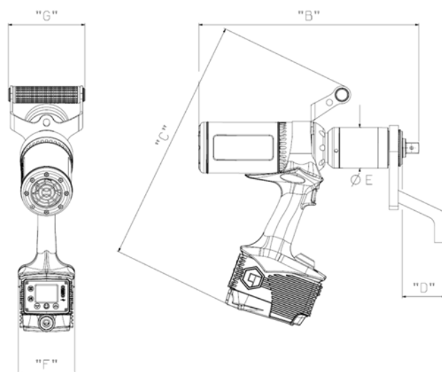
FIGURE 57 – Tool Dimensions
